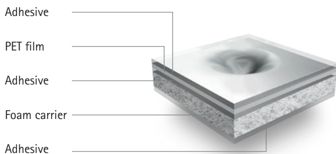
Conventional foam adhesive tape with laminated PET film.
